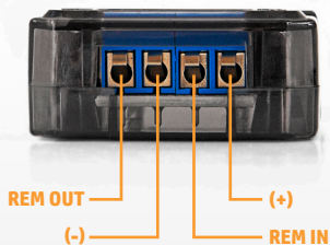
VEX 1.0 | Side |
